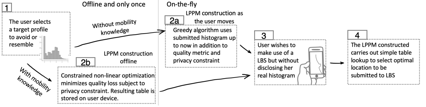
Fig. 2. Illustration of the use of the framework for constructing and using LPPMs.
